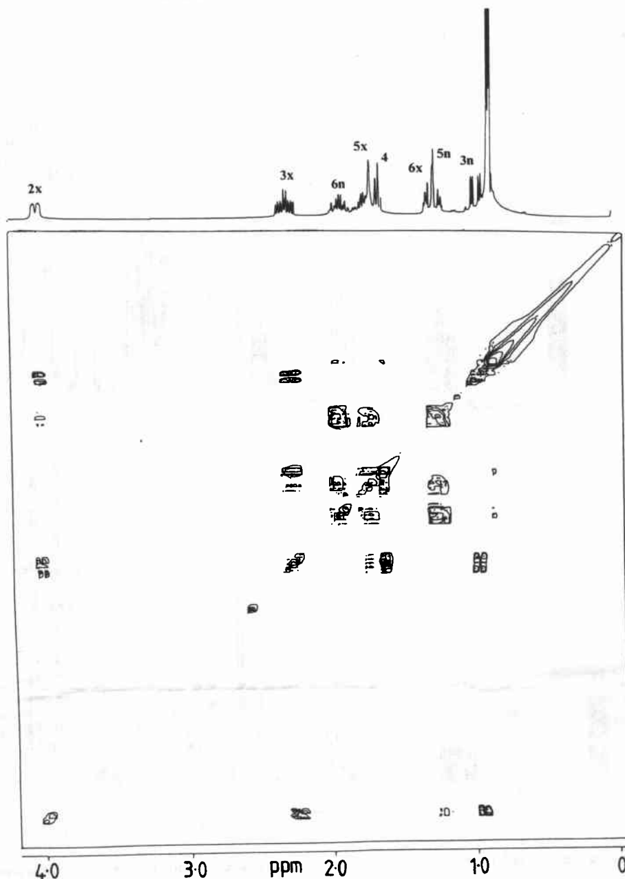
Figure 5. 250-MHz 1 H/ 1 H DQF COSY for 1-borneol.
