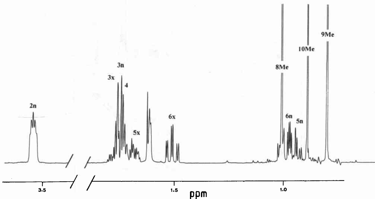
Figure 3. 500-MHz ^1\text{H} NMR spectrum of isborneol.
