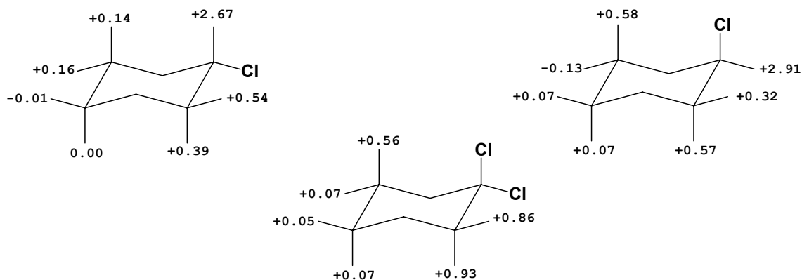
Figure 1 : Experimental (this work) chlorine SCS effects in chloro-cyclohexanes.
